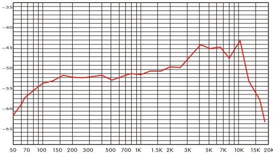
SM-300 Spectrum graph
