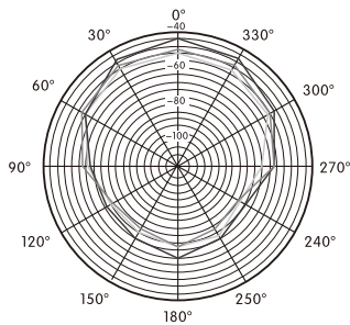
SM-300 Polar Patterns
