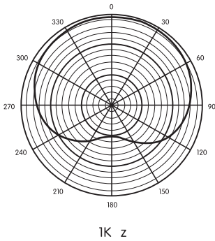
PM-100 Polar Patterns
