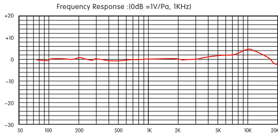
PM-100 Spectrum graph
